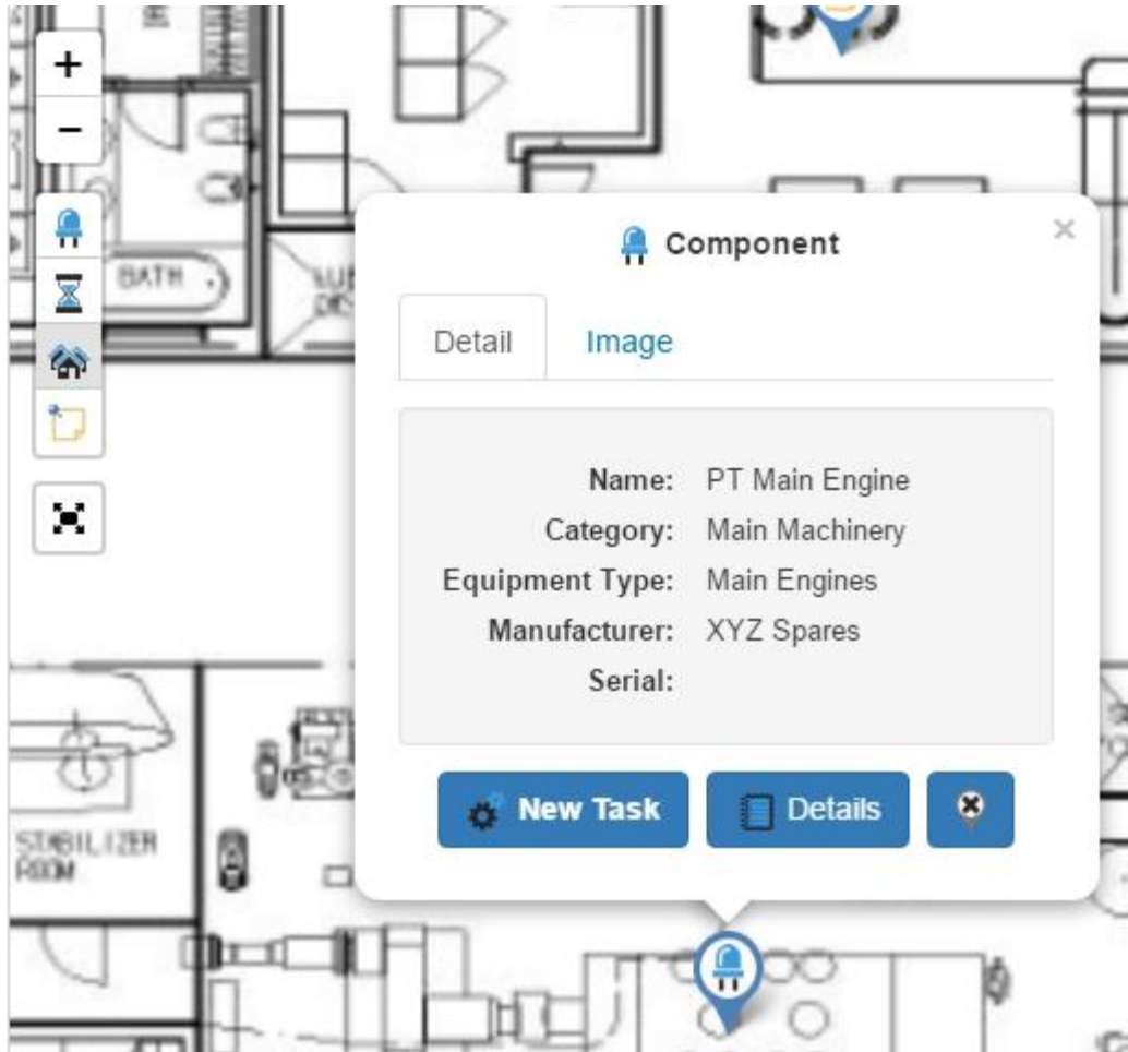
Figure 7 Detail pop-up
